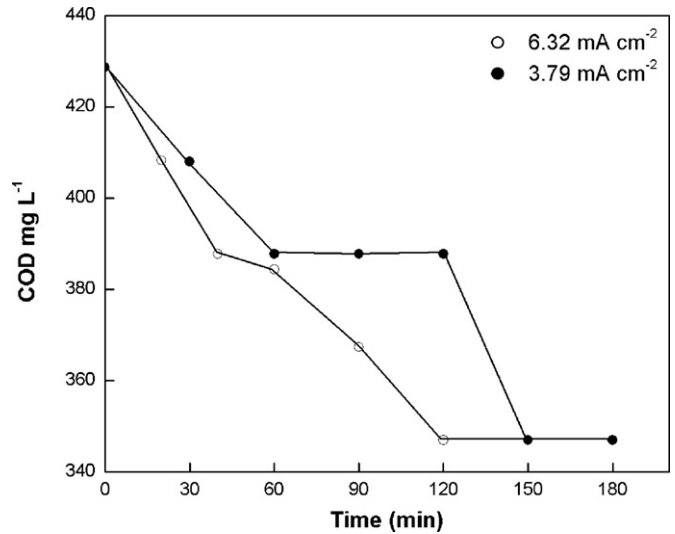
Fig. 7. Effect of current density on COD reduction in the presence of \text{RuO}_2/\text{IrO}_2/\text{TaO}_2 coated titanium.
