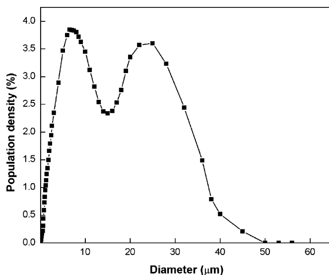
Fig. 2. Distribution of suspended solids in raw sample.
